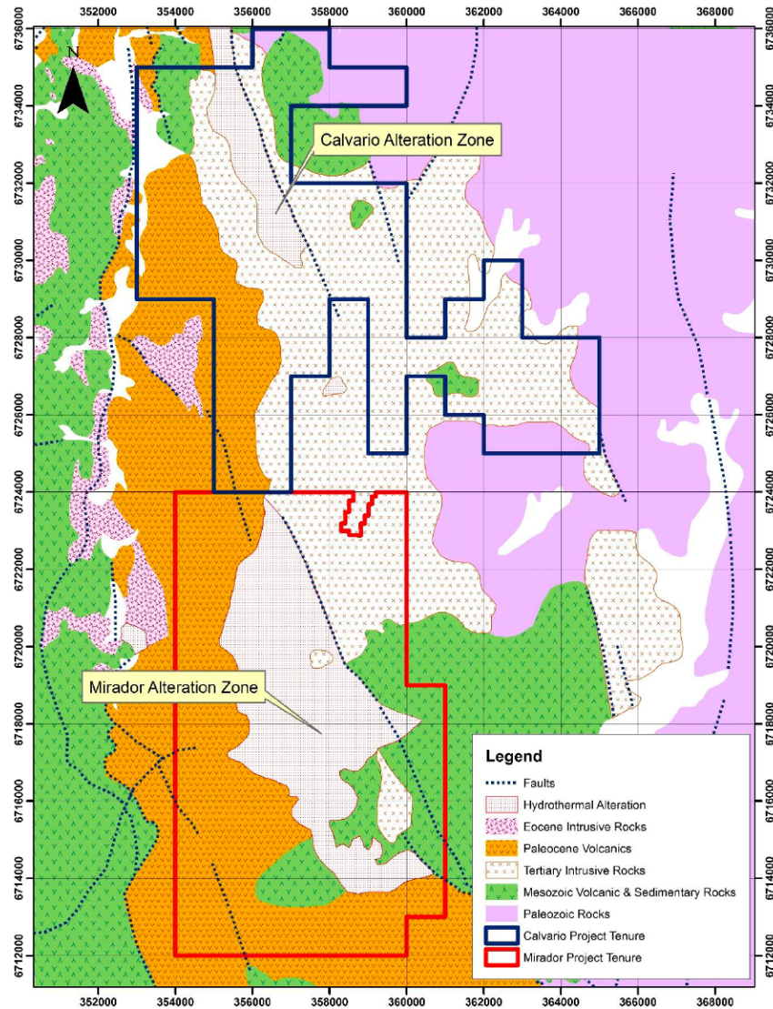
Figure 4: Calvario & Mirador Regional Geology and major copper porphyry related alteration areas.
